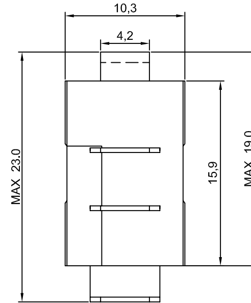
SCHEMATIC
