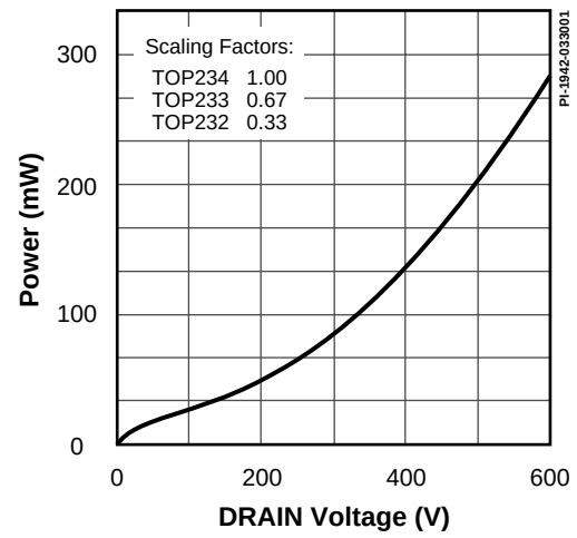
DRAIN CAPACITANCE POWER (132 kHz)
