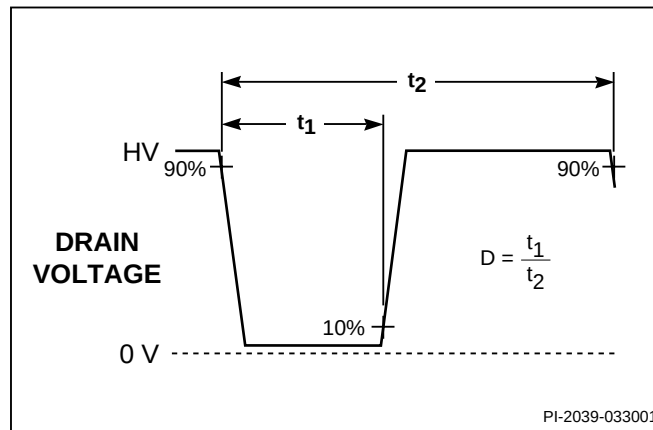
Figure 31. Duty Cycle Measurement.
